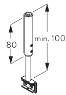
SG 3610 Pendel
