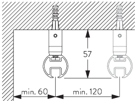
Pendel SG 6175
