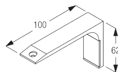
SG 11669 Support design
