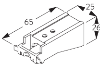
SG 3660 Steun 65 mm
